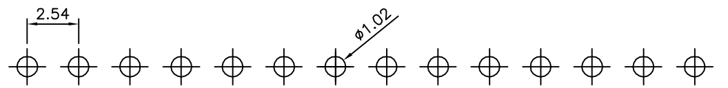
△ Recommended P.C.B. Layout (Top Side) (PCB Board Tolerance ±0.05)
